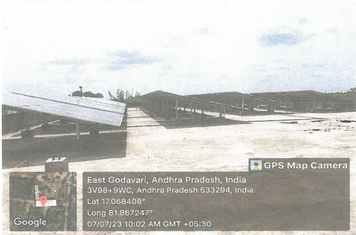
Solar System
