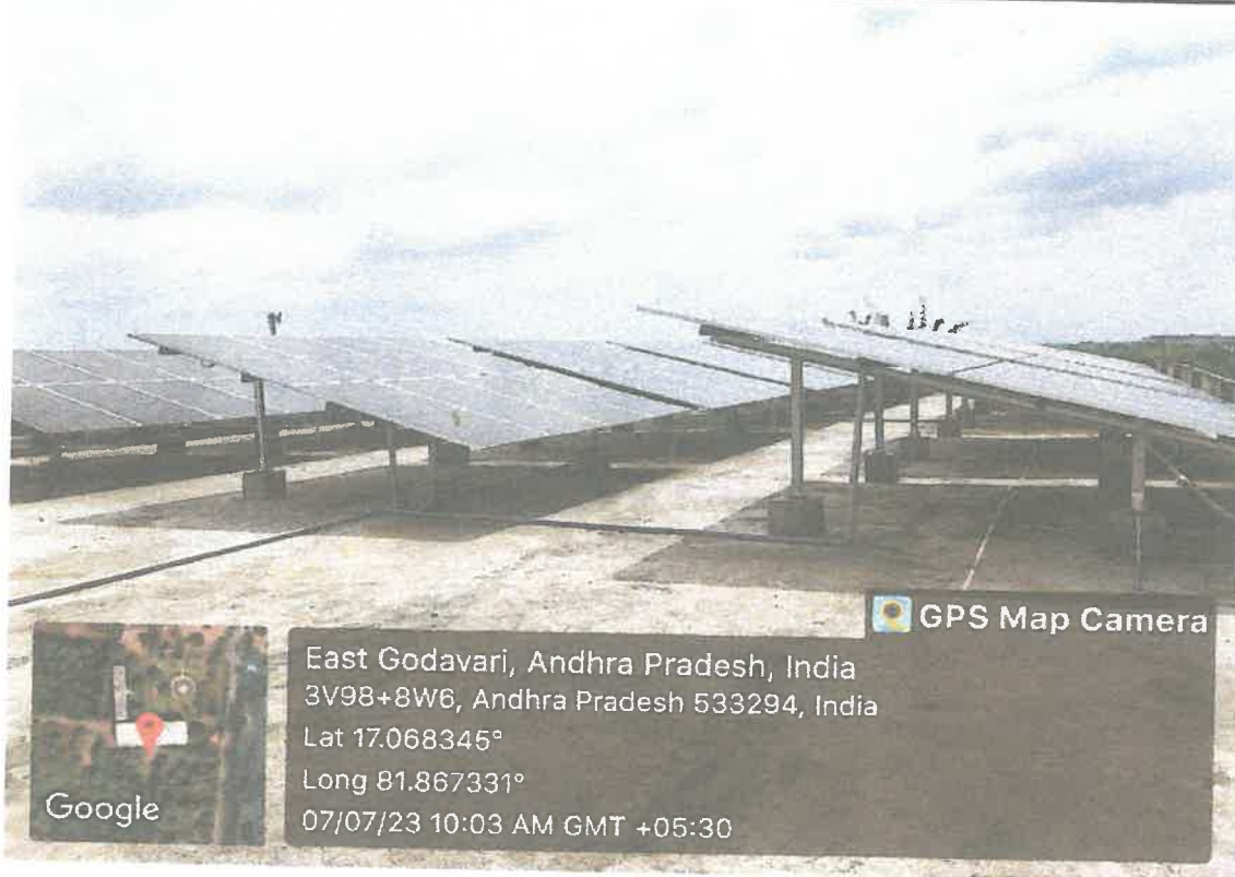
Solar System
