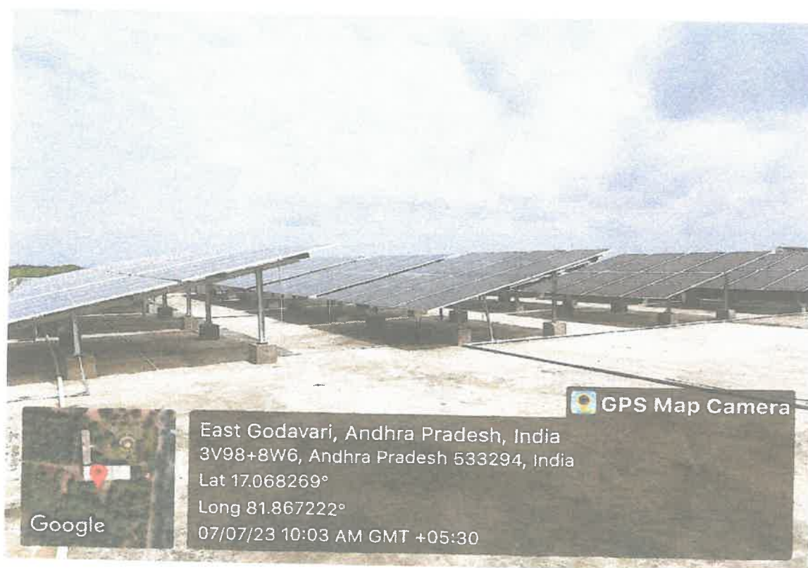
Solar System
